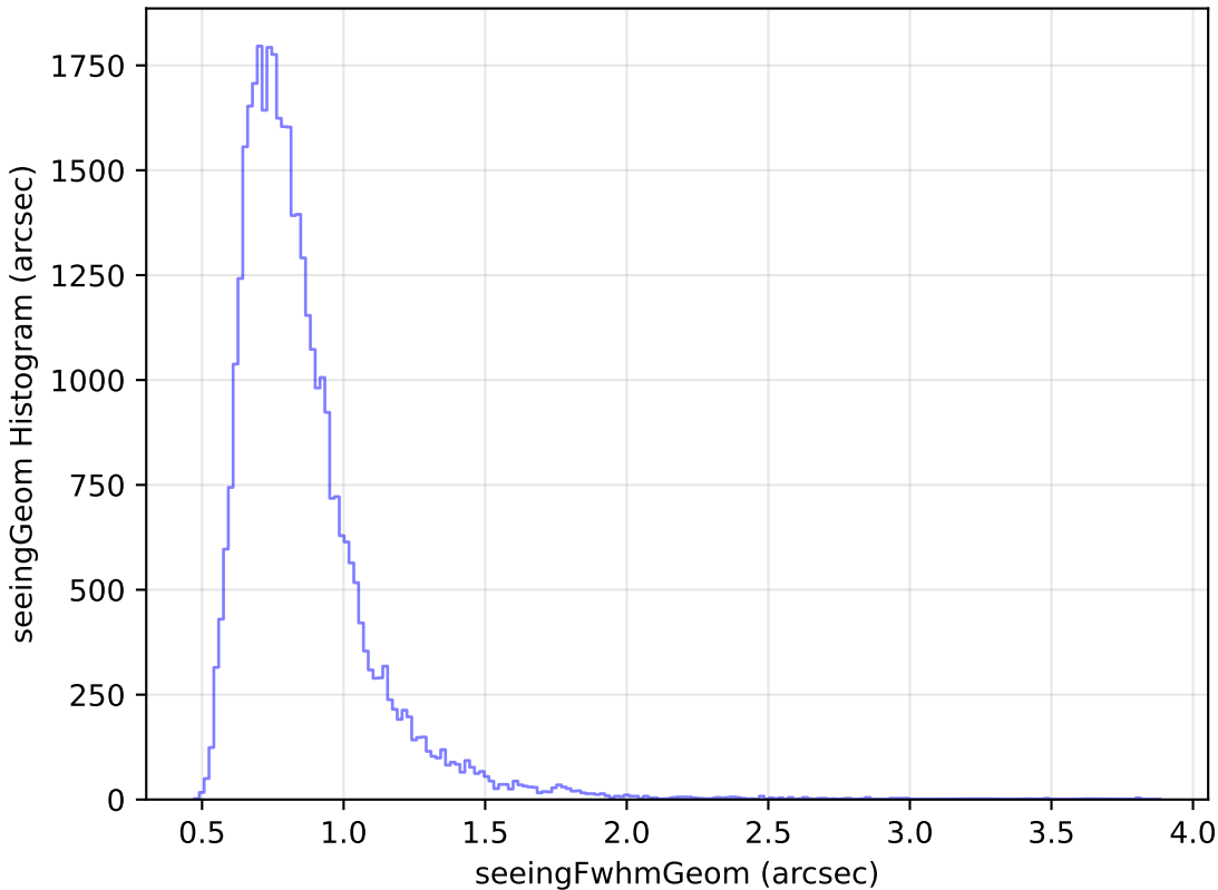
baseline_v3.0_10yrs Yr 1 z band: seeingGeom Histogram
