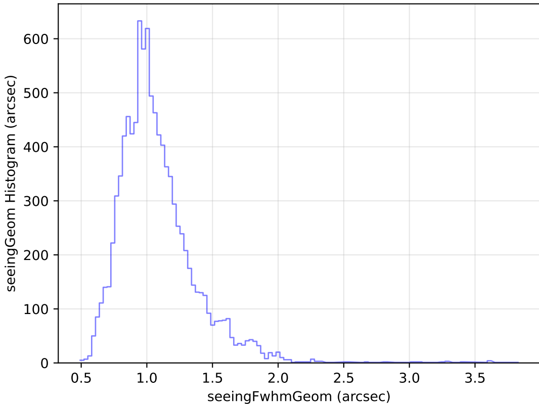
baseline_v3.0_10yrs Yr 1 u band: seeingGeom Histogram
