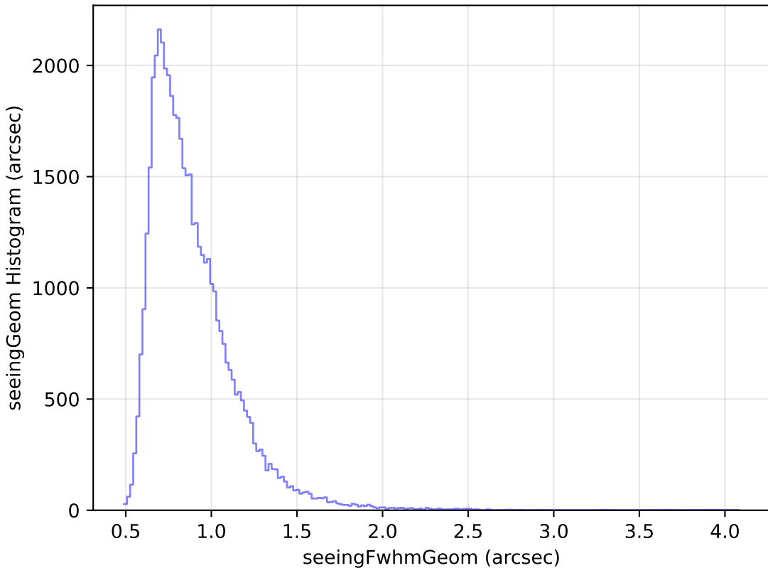
baseline_v3.0_10yrs Yr 1 r band: seeingGeom Histogram
