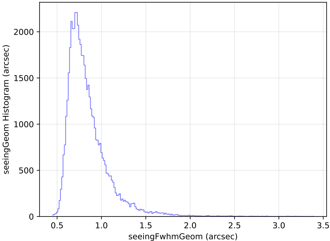
baseline_v3.0_10yrs Yr 1 i band: seeingGeom Histogram
