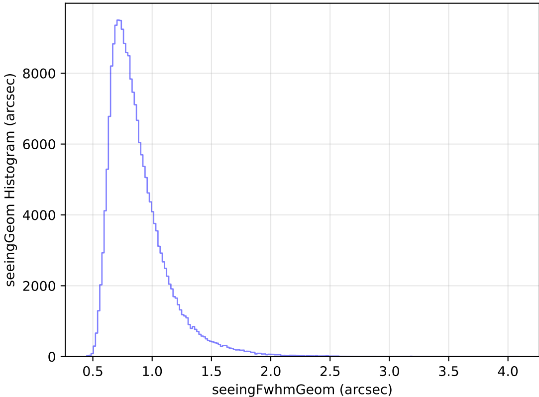
baseline_v3.0_10yrs Yr 1 all bands: seeingGeom Histogram
