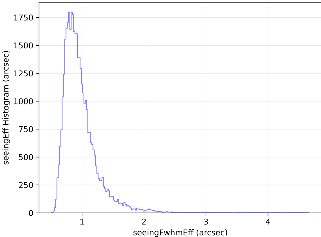
baseline_v3.0_10yrs Yr 1 z band: seeingEff Histogram
