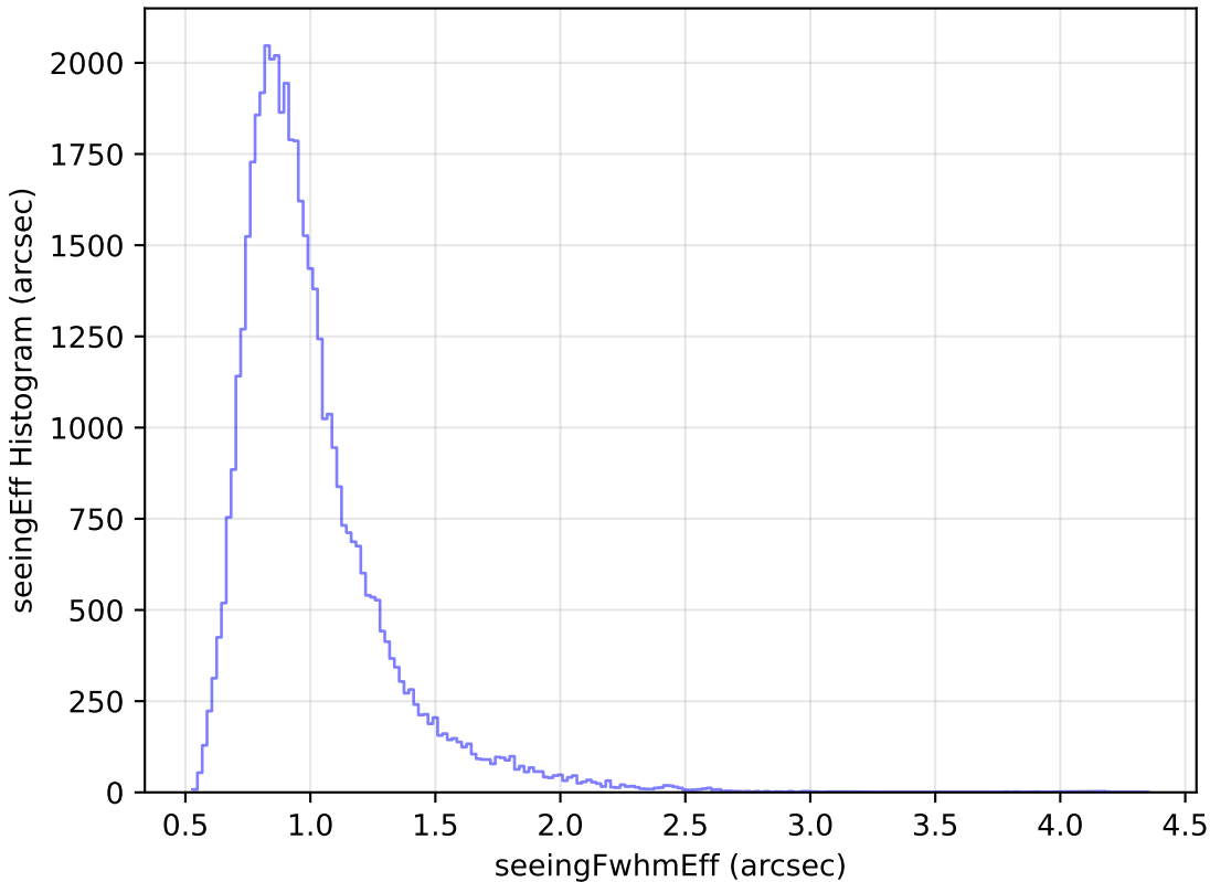
baseline_v3.0_10yrs Yr 1 y band: seeingEff Histogram
