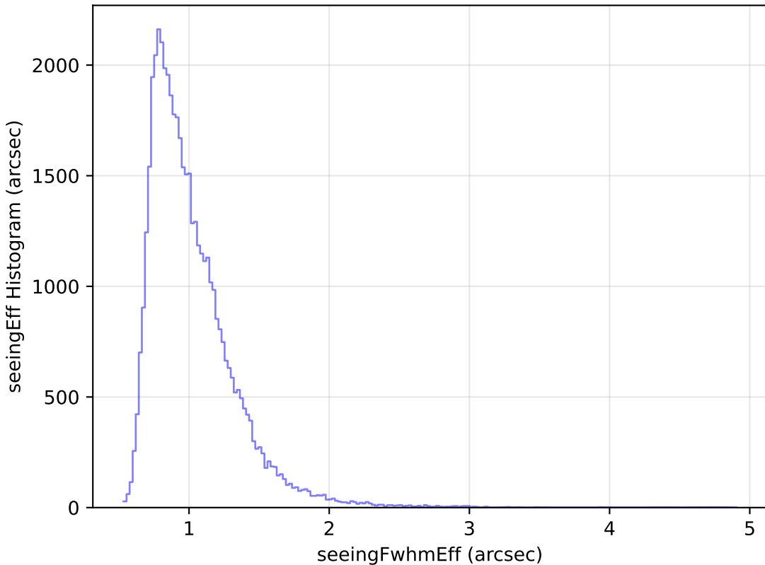
baseline_v3.0_10yrs Yr 1 r band: seeingEff Histogram
