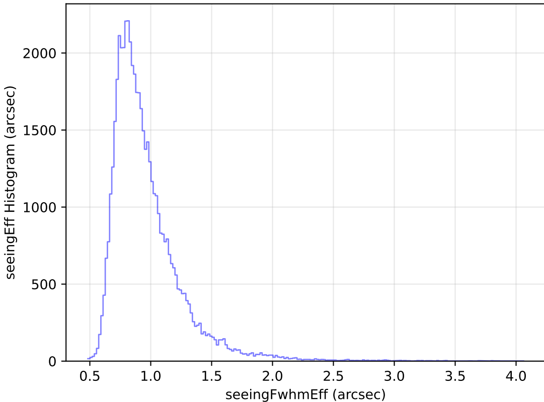
baseline_v3.0_10yrs Yr 1 i band: seeingEff Histogram
