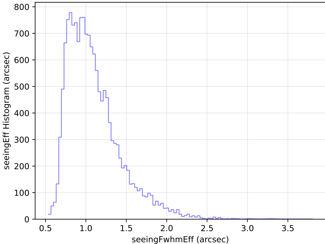
baseline_v3.0_10yrs Yr 1 g band: seeingEff Histogram
