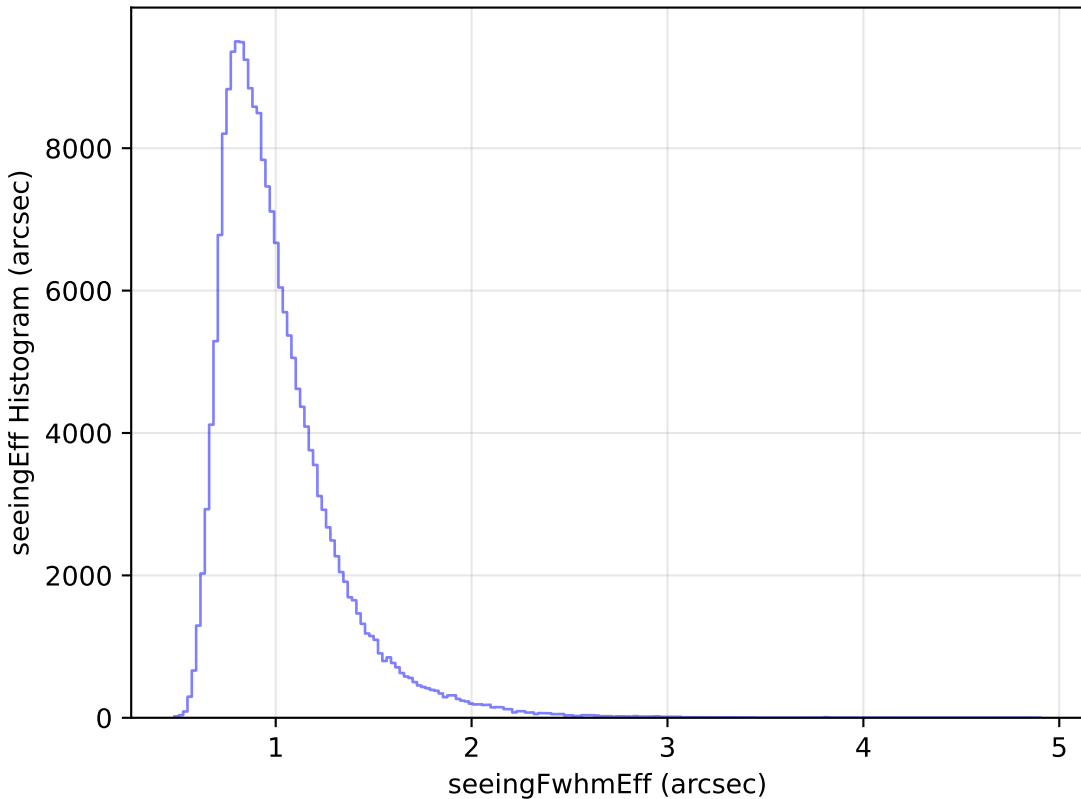
baseline_v3.0_10yrs Yr 1 all bands: seeingEff Histogram
