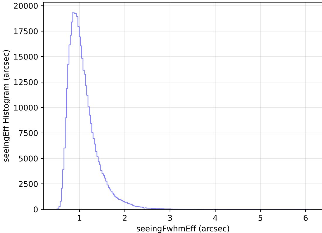
baseline_v3.0_10yrs WFD z band: seeingEff Histogram
