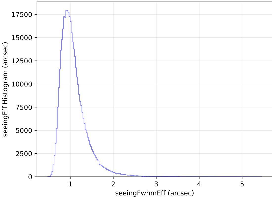
baseline_v3.0_10yrs WFD y band: seeingEff Histogram
