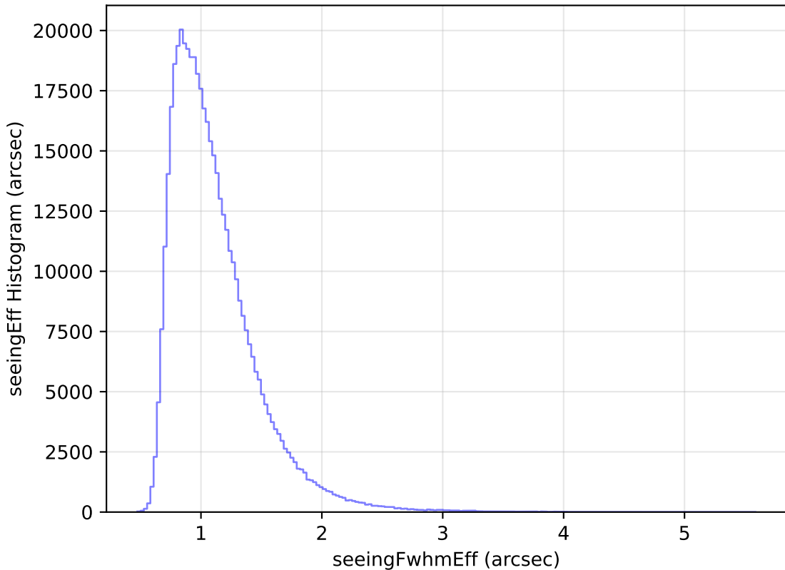
baseline_v3.0_10yrs WFD r band: seeingEff Histogram
