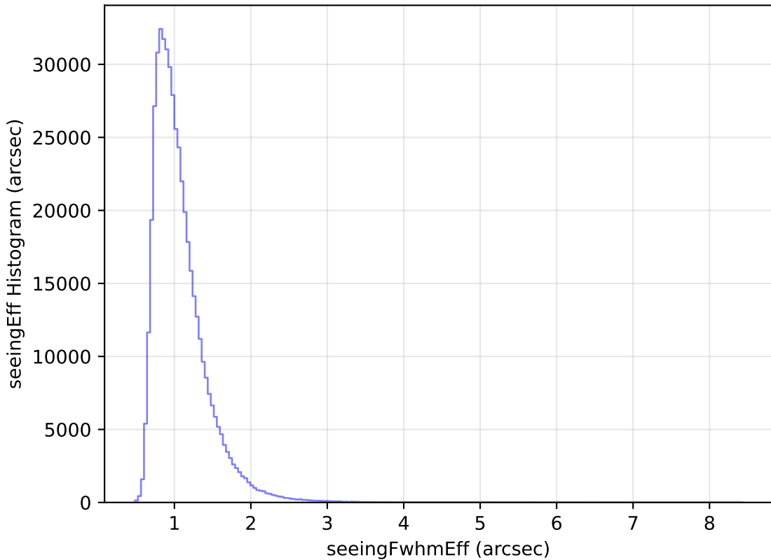
baseline_v3.0_10yrs WFD i band: seeingEff Histogram
