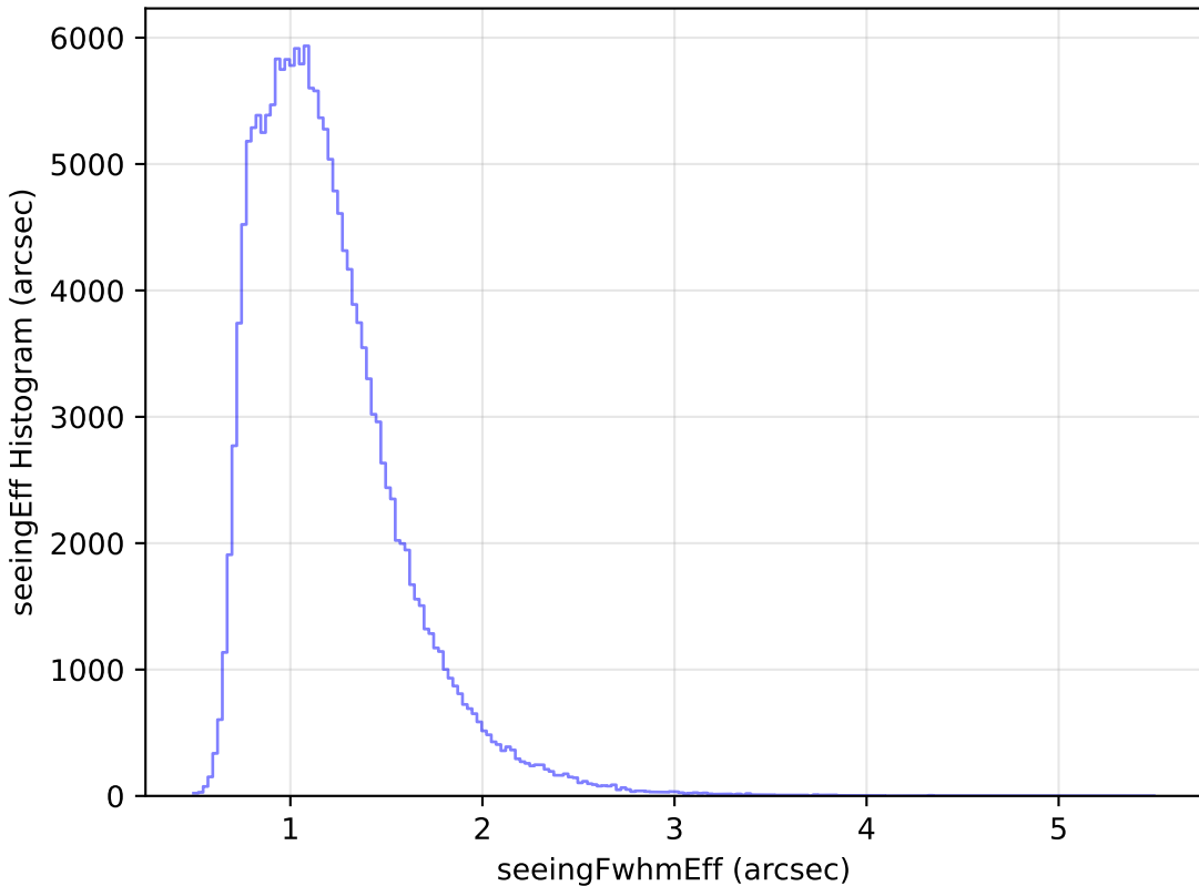
baseline_v3.0_10yrs WFD g band: seeingEff Histogram
