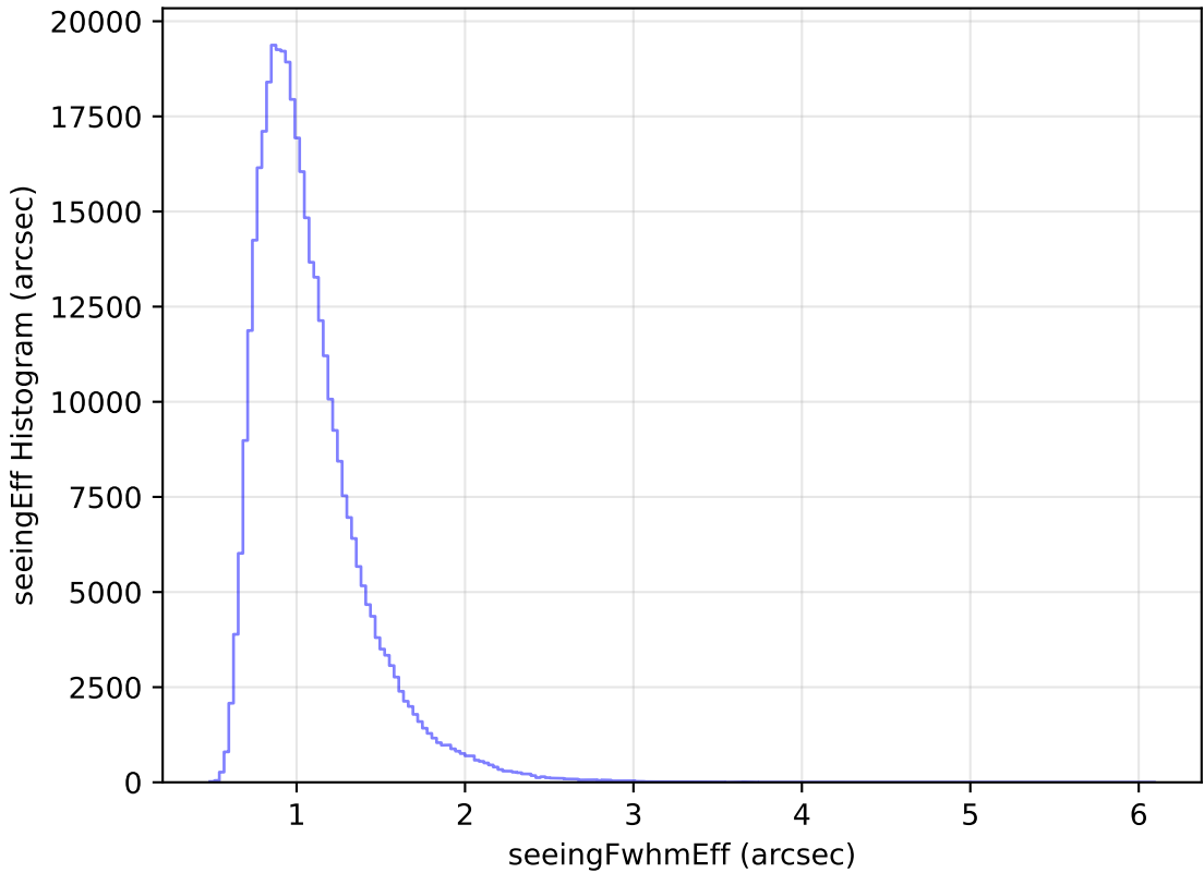
baseline_v3.0_10yrs All sky z band: seeingEff Histogram
