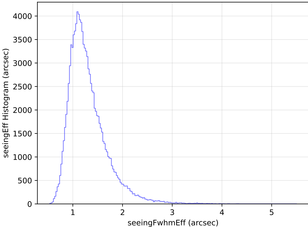
baseline_v3.0_10yrs All sky u band: seeingEff Histogram
