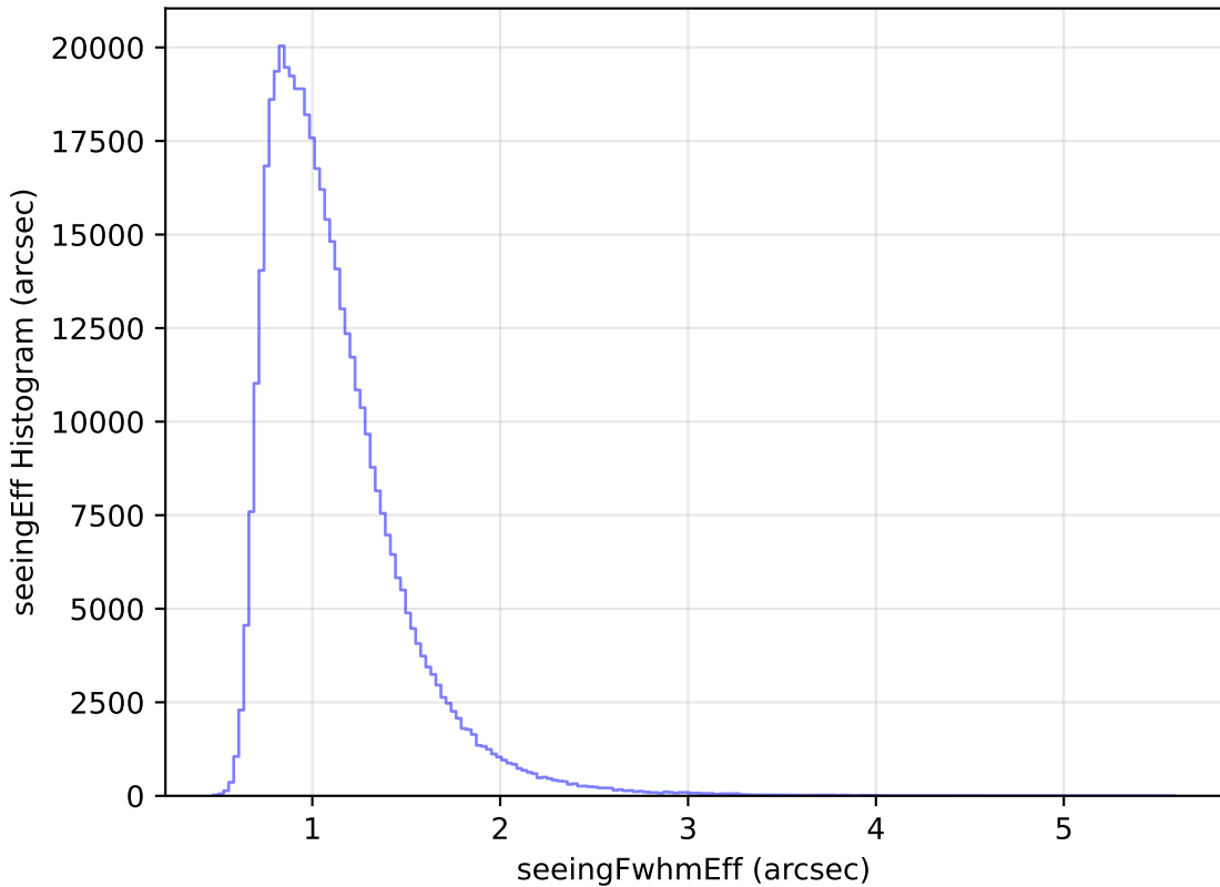
baseline_v3.0_10yrs All sky r band: seeingEff Histogram
