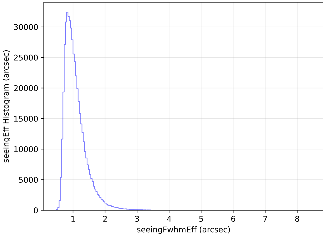
baseline_v3.0_10yrs All sky i band: seeingEff Histogram
