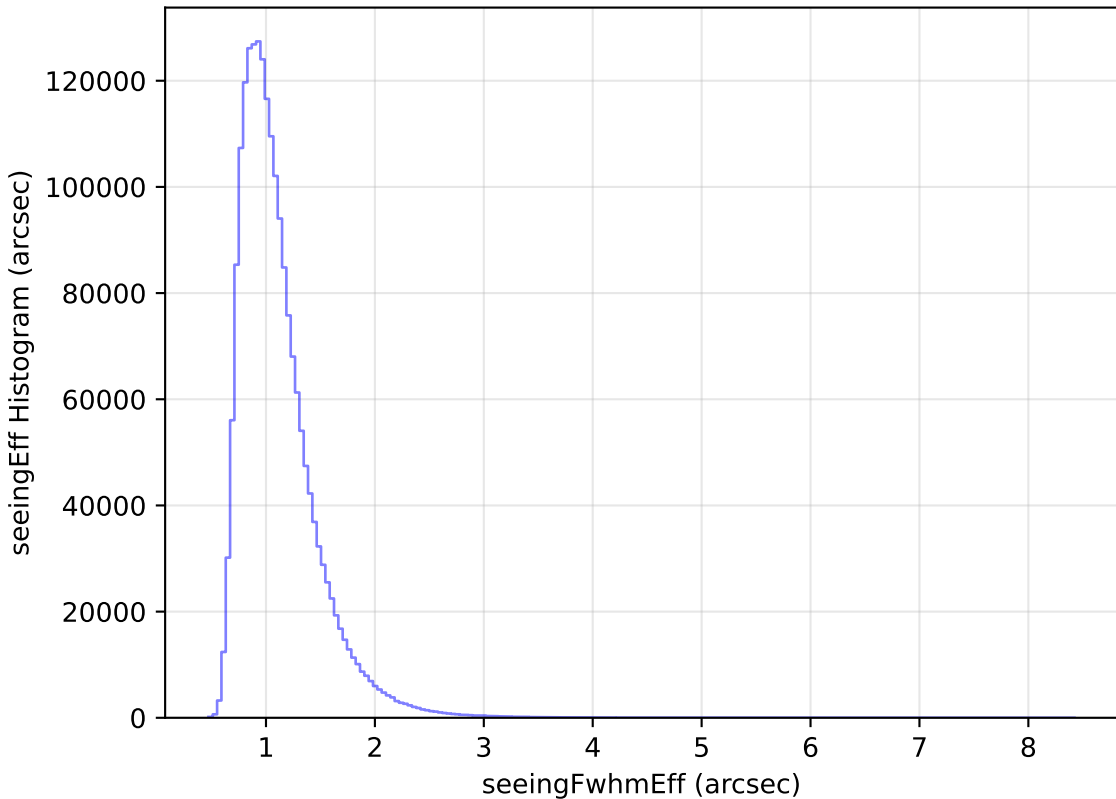
baseline_v3.0_10yrs All sky all bands: seeingEff Histogram
