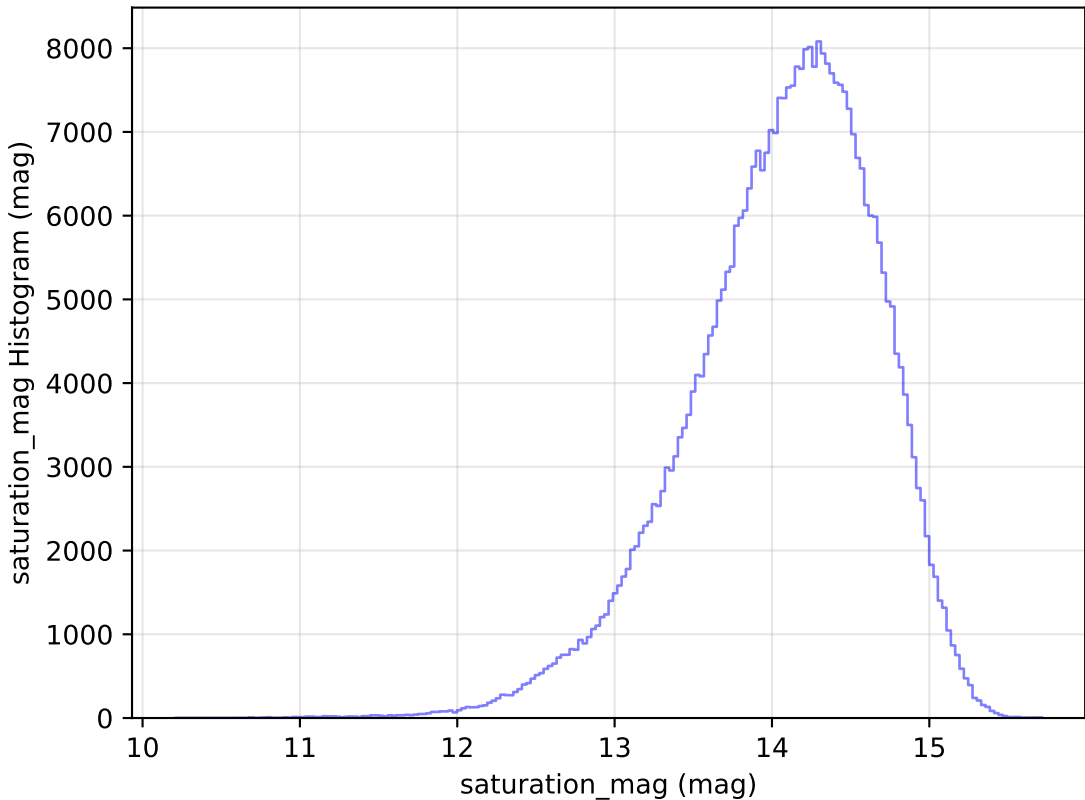
baseline_v3.0_10yrs WFD z band: saturation_mag Histogram
