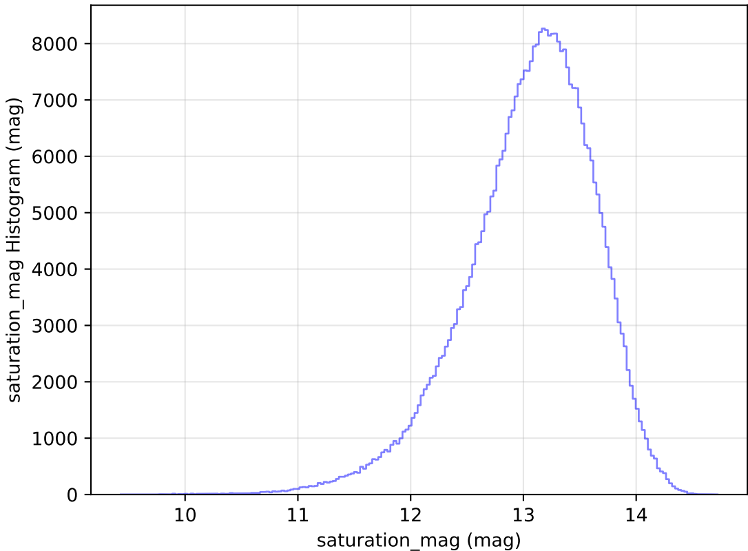
baseline_v3.0_10yrs WFD y band: saturation_mag Histogram
