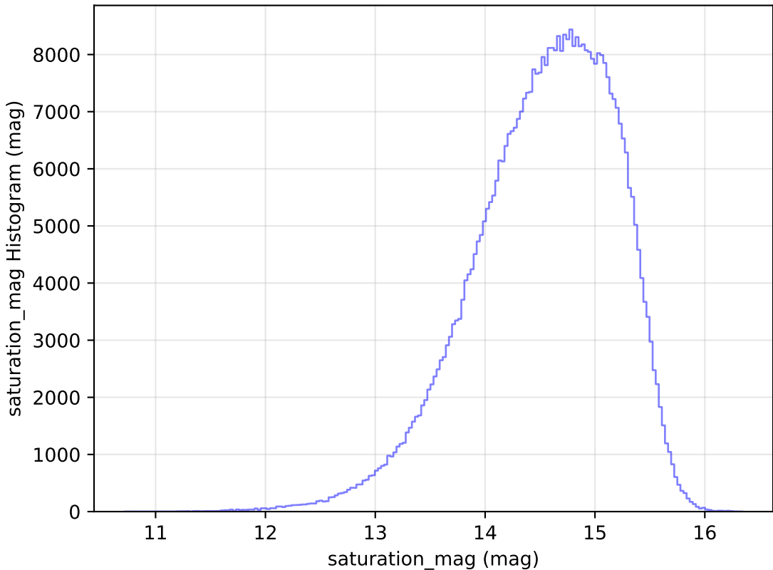
baseline_v3.0_10yrs WFD r band: saturation_mag Histogram
