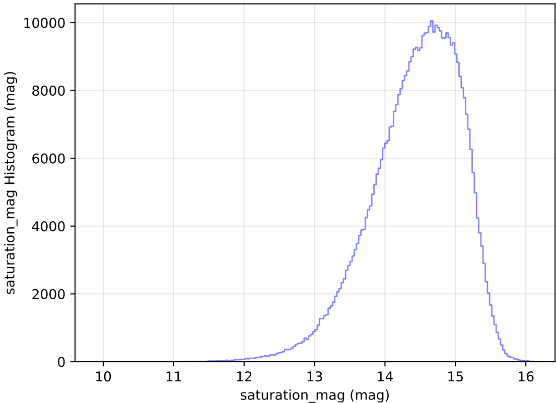
baseline_v3.0_10yrs WFD i band: saturation_mag Histogram
