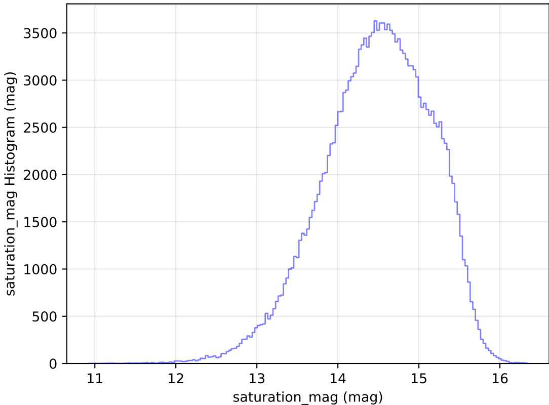
baseline_v3.0_10yrs WFD g band: saturation_mag Histogram
