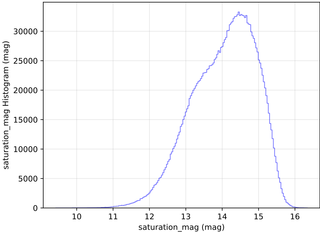
baseline_v3.0_10yrs WFD all bands: saturation_mag Histogram
