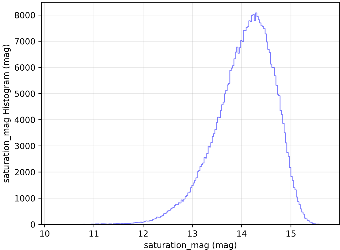
baseline_v3.0_10yrs All sky z band: saturation_mag Histogram
