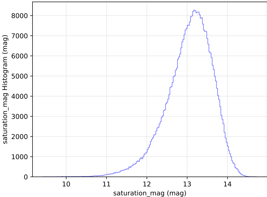
baseline_v3.0_10yrs All sky y band: saturation_mag Histogram
