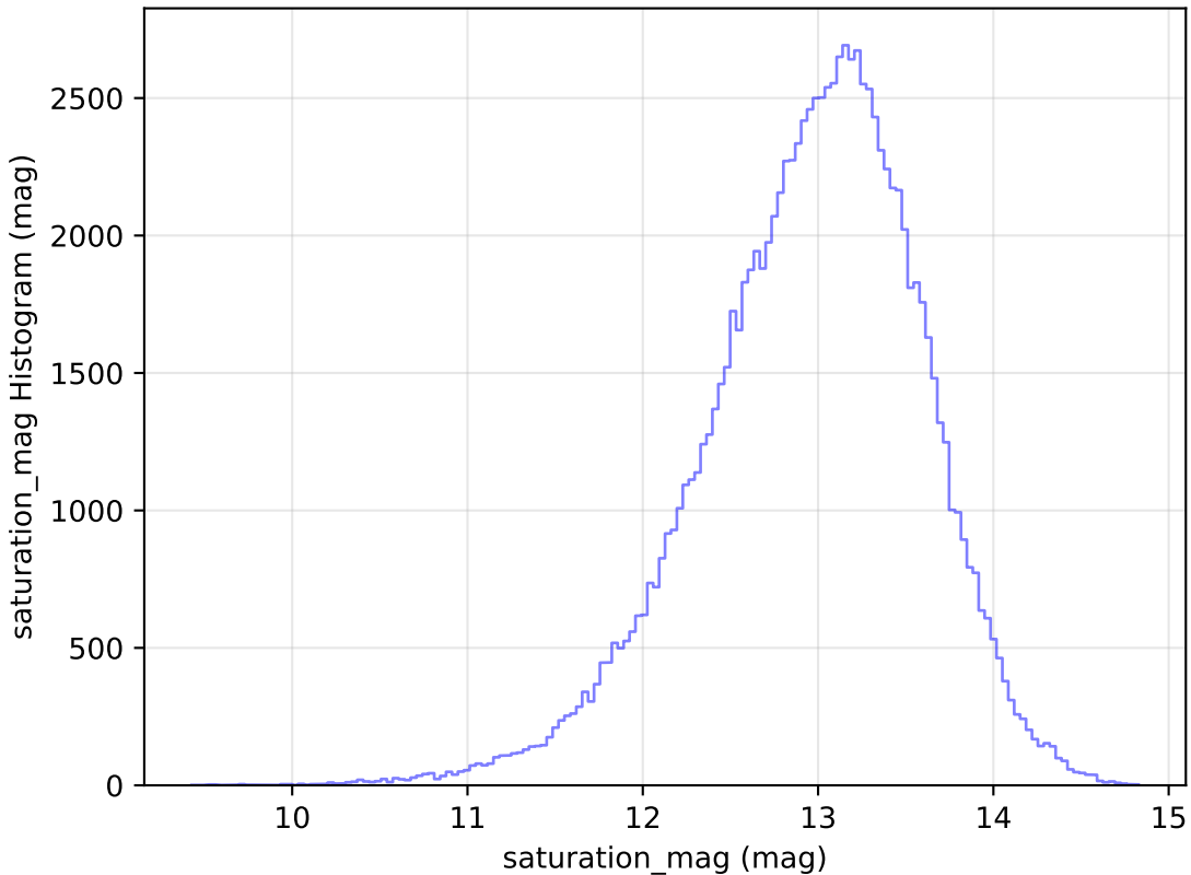
baseline_v3.0_10yrs All sky u band: saturation_mag Histogram
