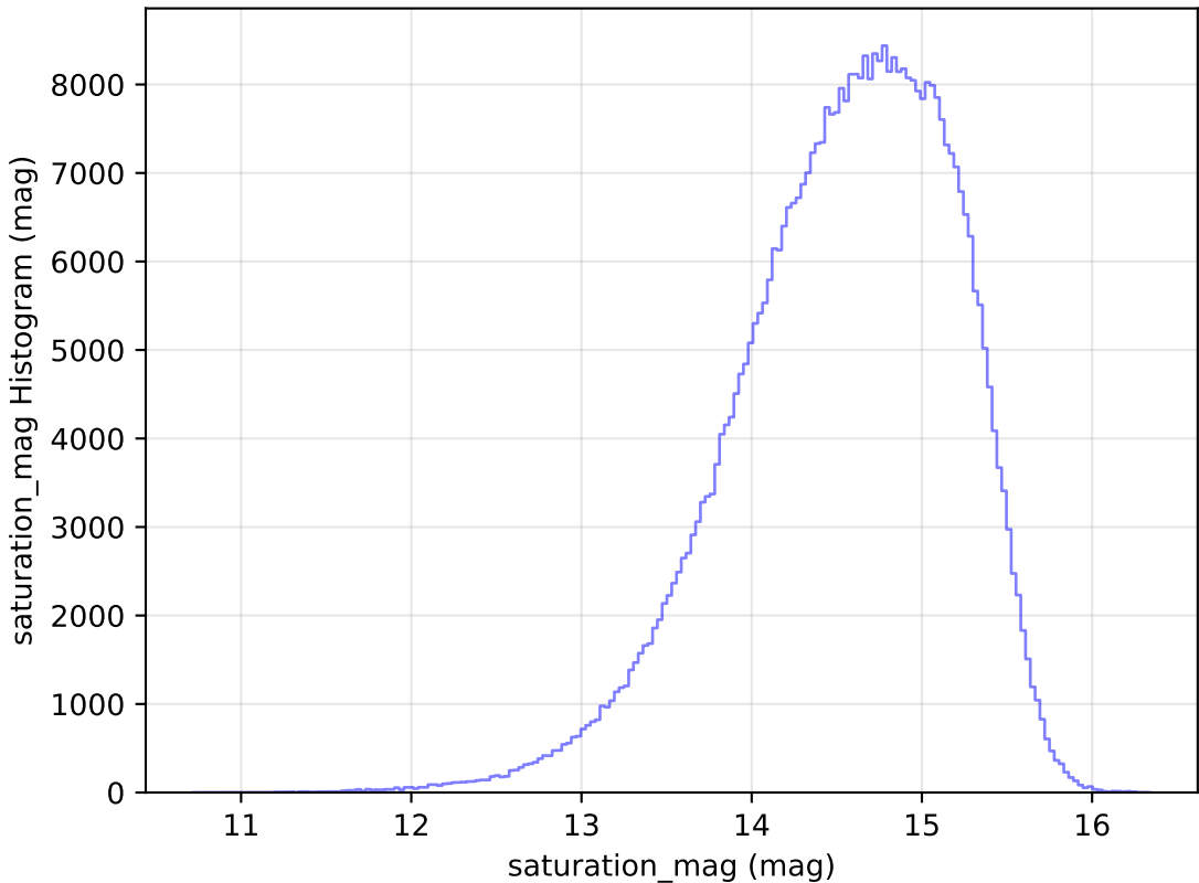
baseline_v3.0_10yrs All sky r band: saturation_mag Histogram
