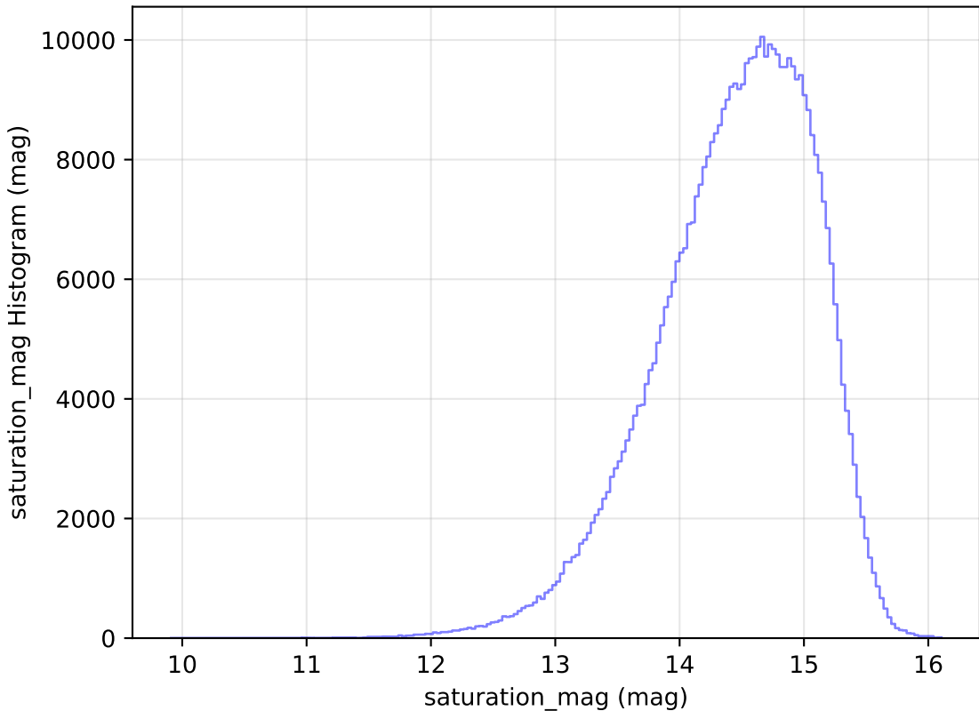
baseline_v3.0_10yrs All sky i band: saturation_mag Histogram
