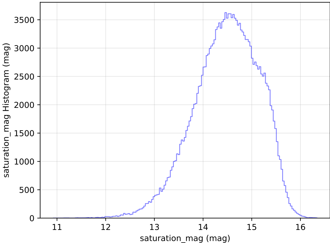
baseline_v3.0_10yrs All sky g band: saturation_mag Histogram
