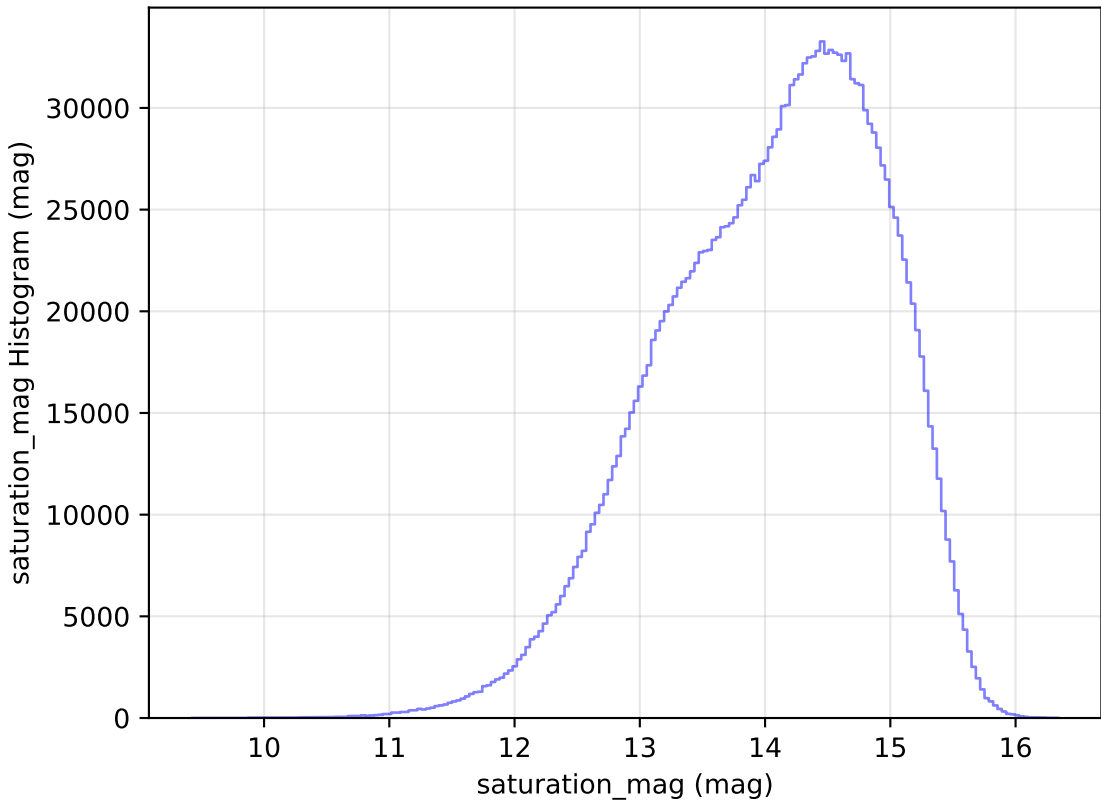
baseline_v3.0_10yrs All sky all bands: saturation_mag Histogram
