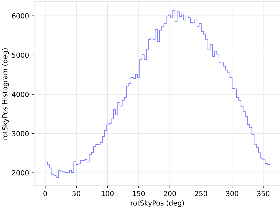
baseline_v3.0_10yrs WFD z band: rotSkyPos Histogram
