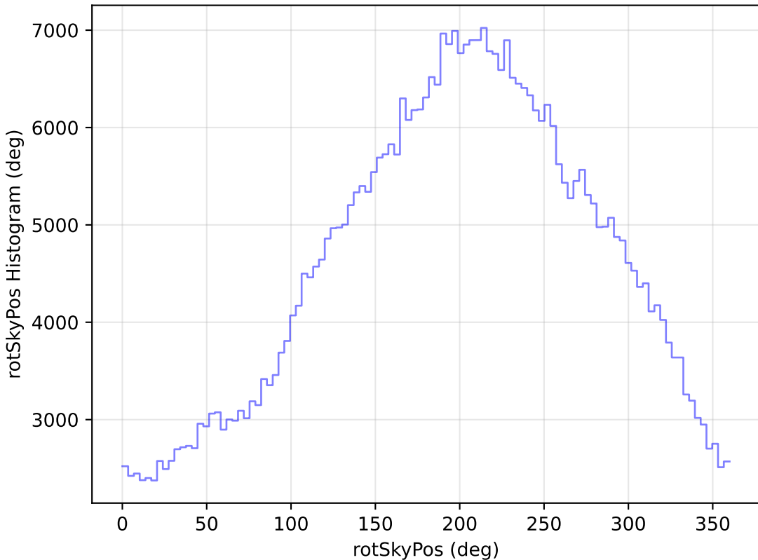
baseline_v3.0_10yrs WFD r band: rotSkyPos Histogram
