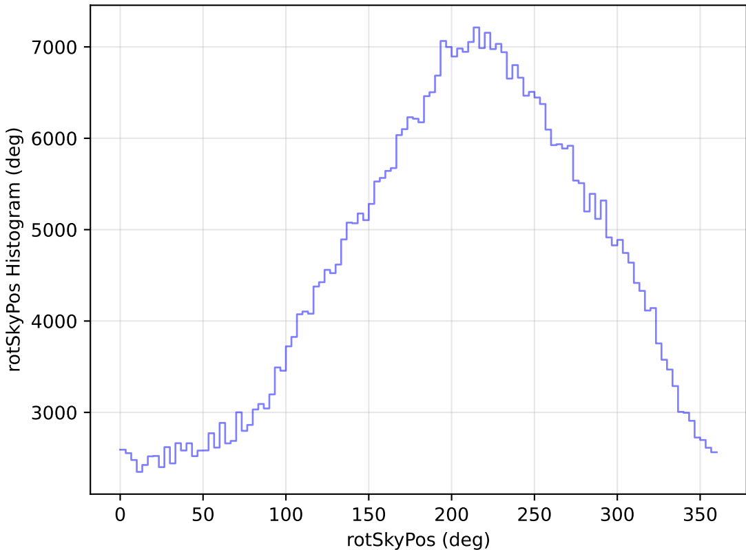
baseline_v3.0_10yrs WFD i band: rotSkyPos Histogram
