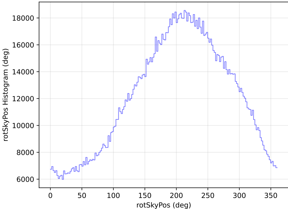
baseline_v3.0_10yrs WFD all bands: rotSkyPos Histogram
