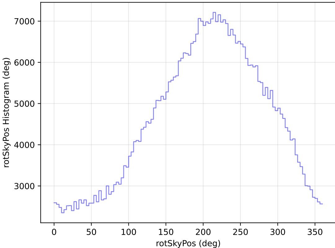
baseline_v3.0_10yrs All sky i band: rotSkyPos Histogram
