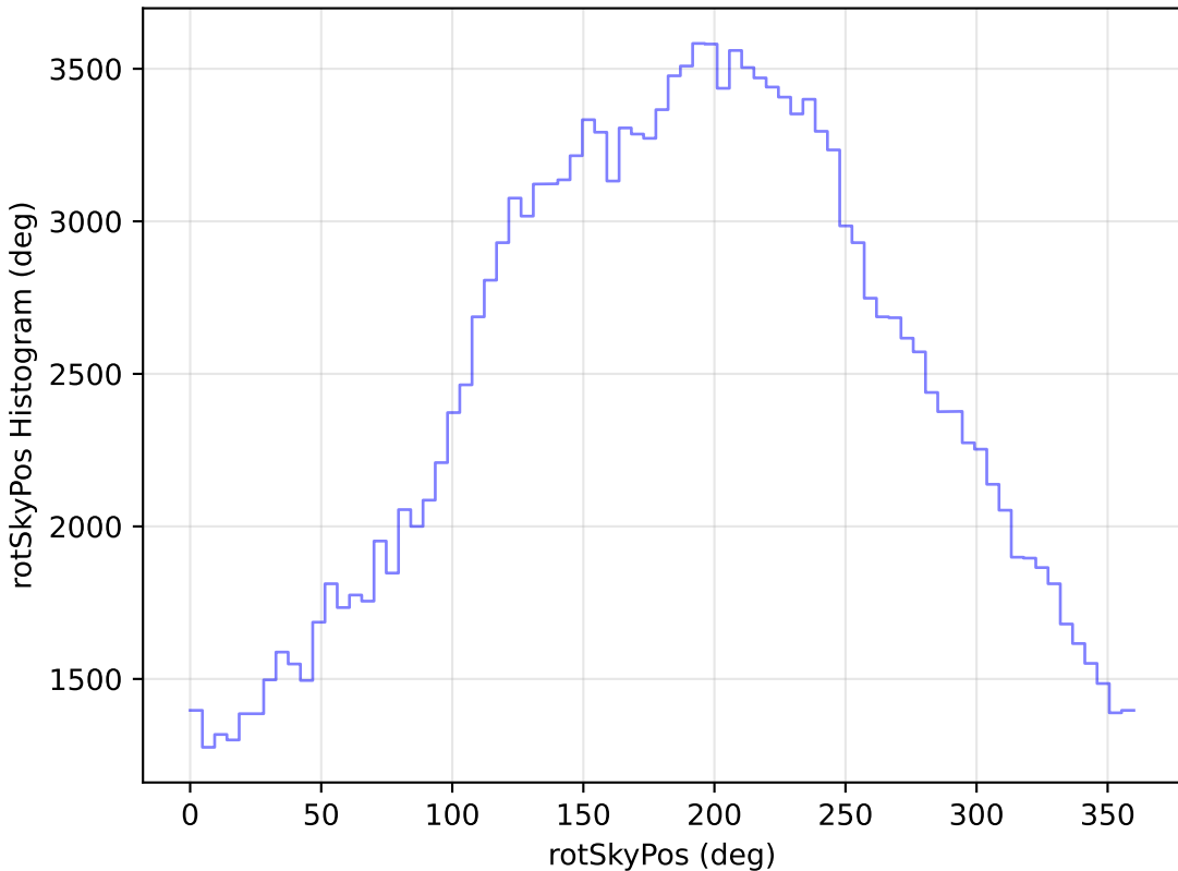
baseline_v3.0_10yrs All sky g band: rotSkyPos Histogram
