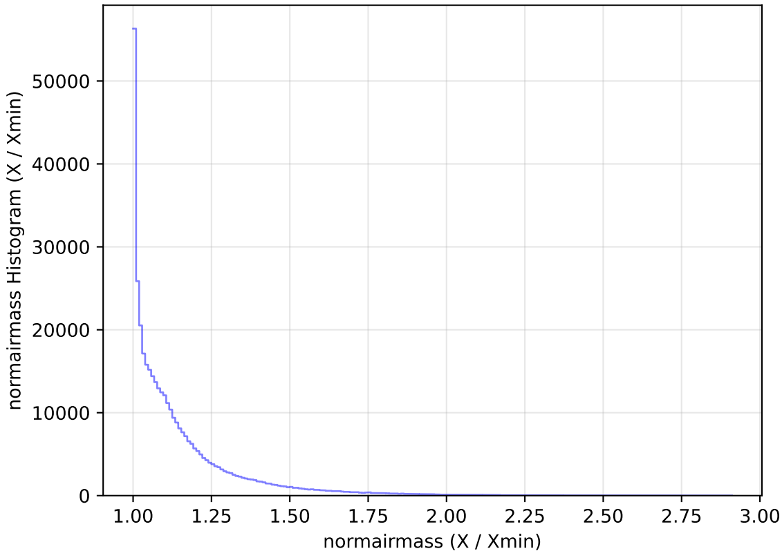
baseline_v3.0_10yrs WFD y band: normairmass Histogram
