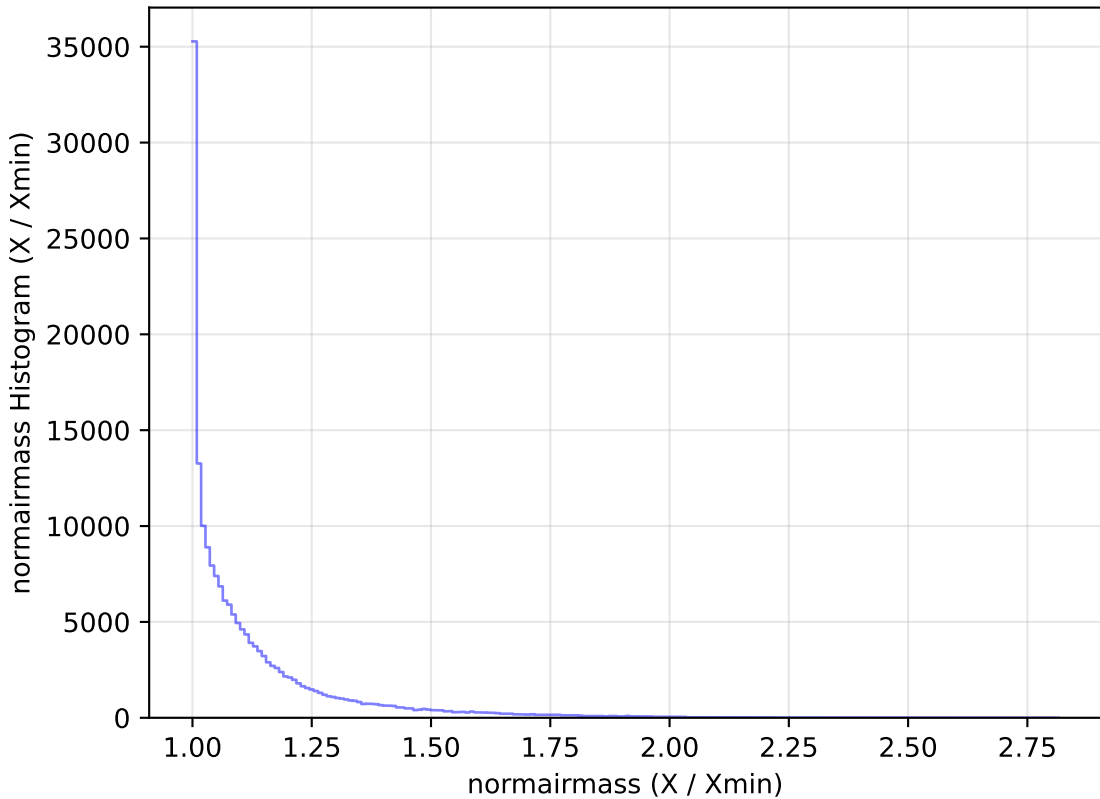
baseline_v3.0_10yrs WFD g band: normairmass Histogram
