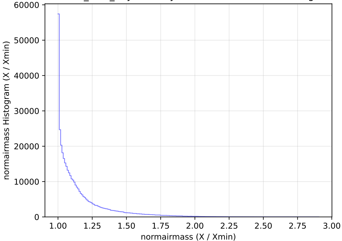
baseline_v3.0_10yrs All sky z band: normairmass Histogram
