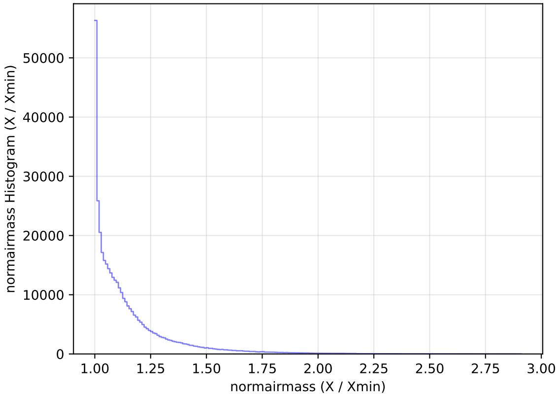
baseline_v3.0_10yrs All sky y band: normairmass Histogram
