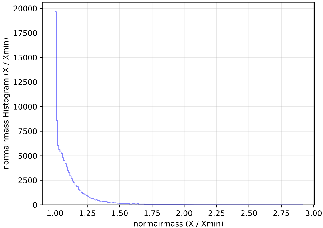
baseline_v3.0_10yrs All sky u band: normairmass Histogram
