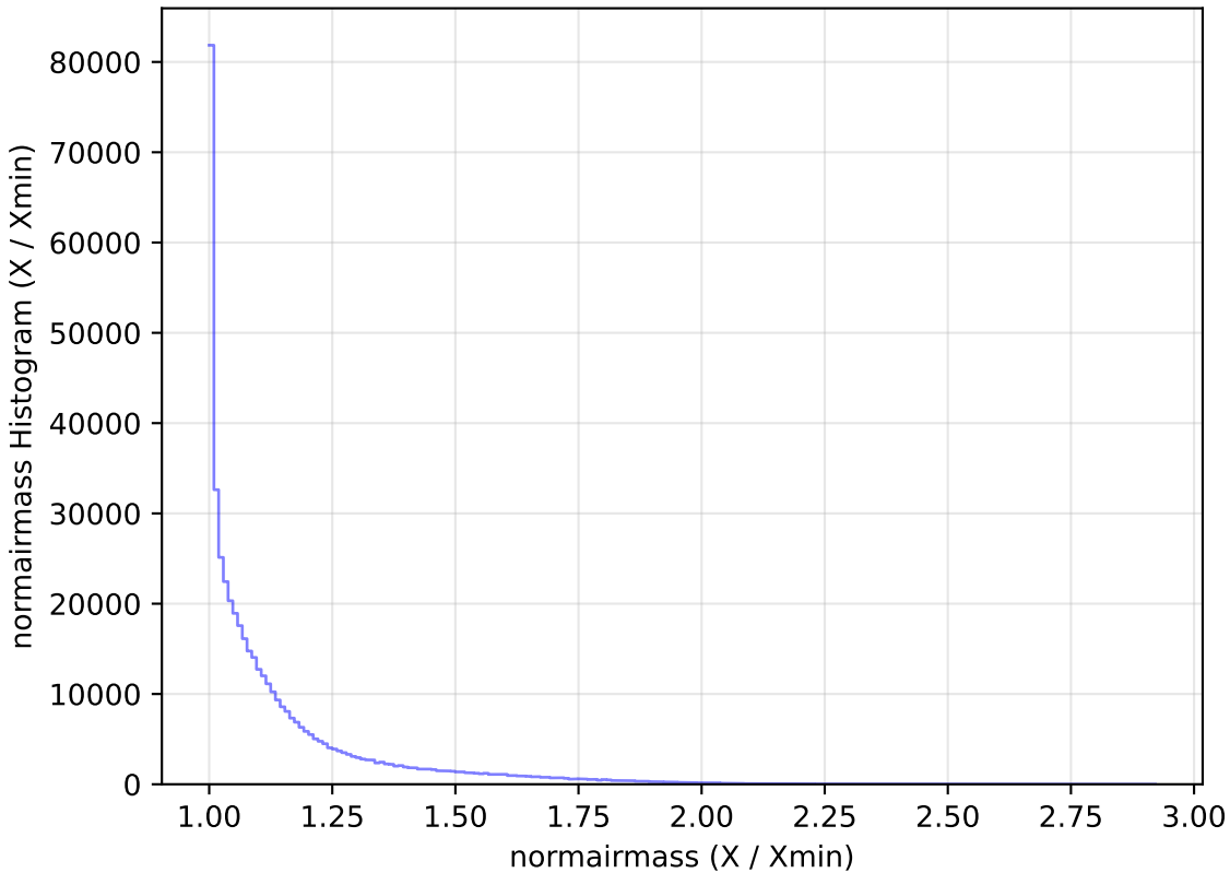
baseline_v3.0_10yrs All sky r band: normairmass Histogram
