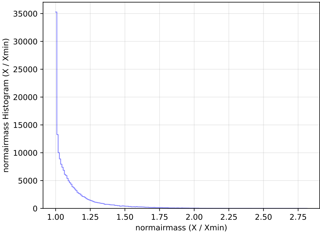
baseline_v3.0_10yrs All sky g band: normairmass Histogram
