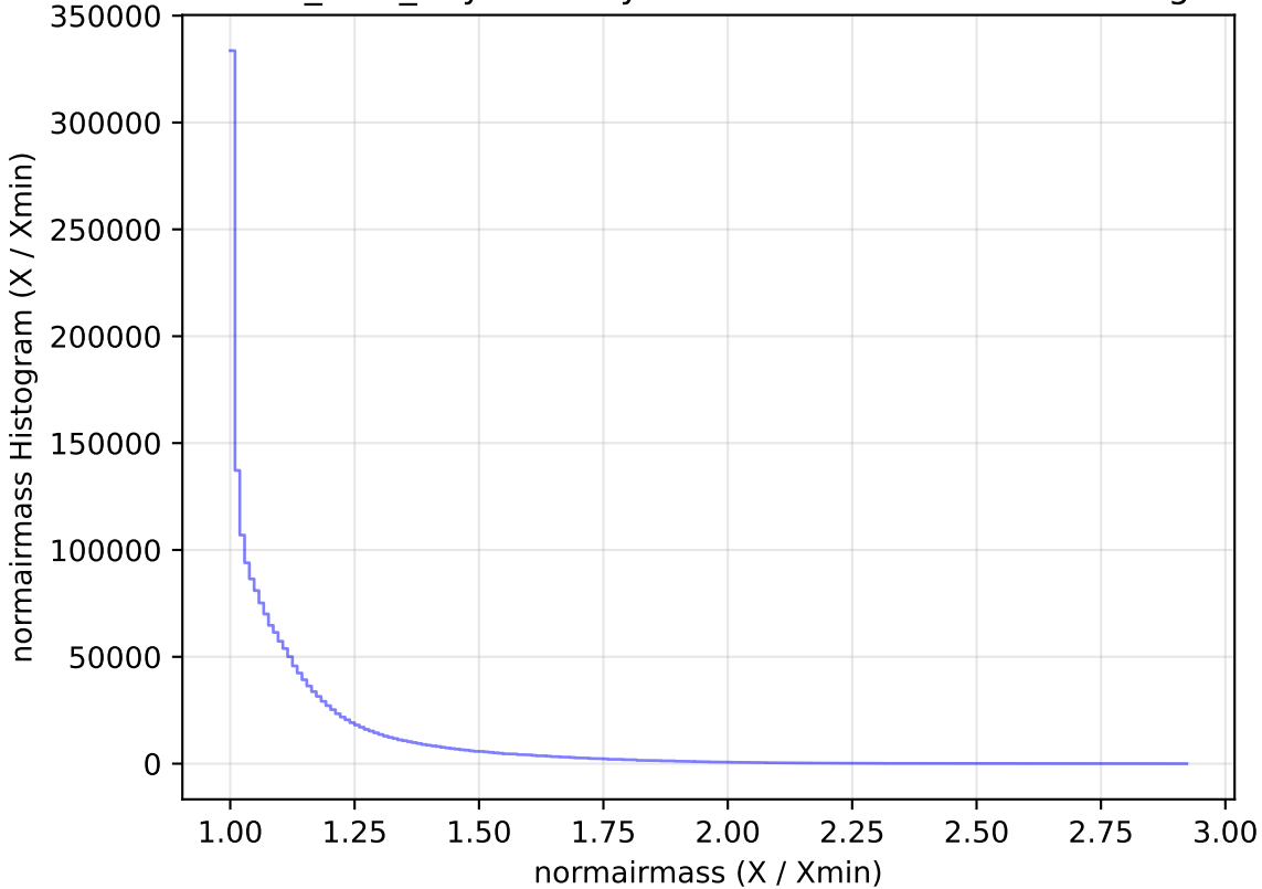
baseline_v3.0_10yrs All sky all bands: normairmass Histogram
