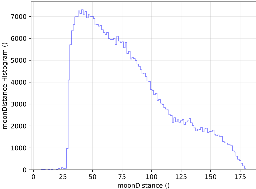
baseline_v3.0_10yrs WFD y band: moonDistance Histogram
