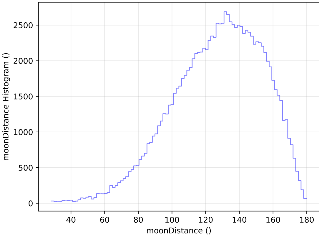
baseline_v3.0_10yrs WFD u band: moonDistance Histogram
